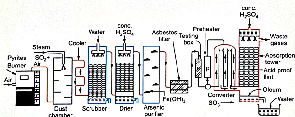
Manufacture of Sulphuric acid by Contact process
